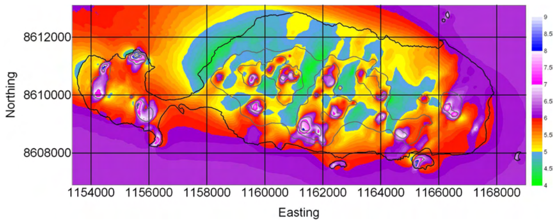
Figure 6.17: Windmap for 50m anemometer height. This wind map is based on data for all of 2003.
