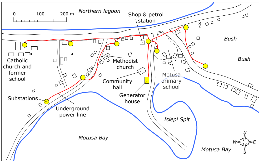
Figure 5.14: Map of the electricity grid in Motusa. Motusa features the largest village grid on Rotuma.
