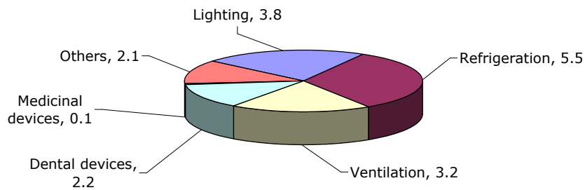
Figure 5.31: Energy use in Rotuma hospital. All values are in kWh per day.
