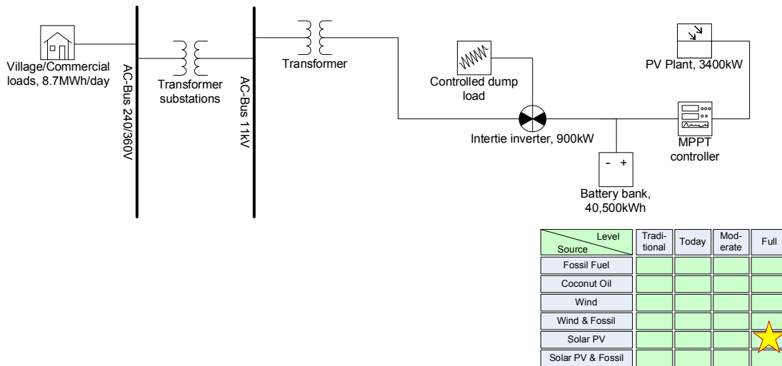
Figure 7.25: Level D: Solar PV generation scheme.
