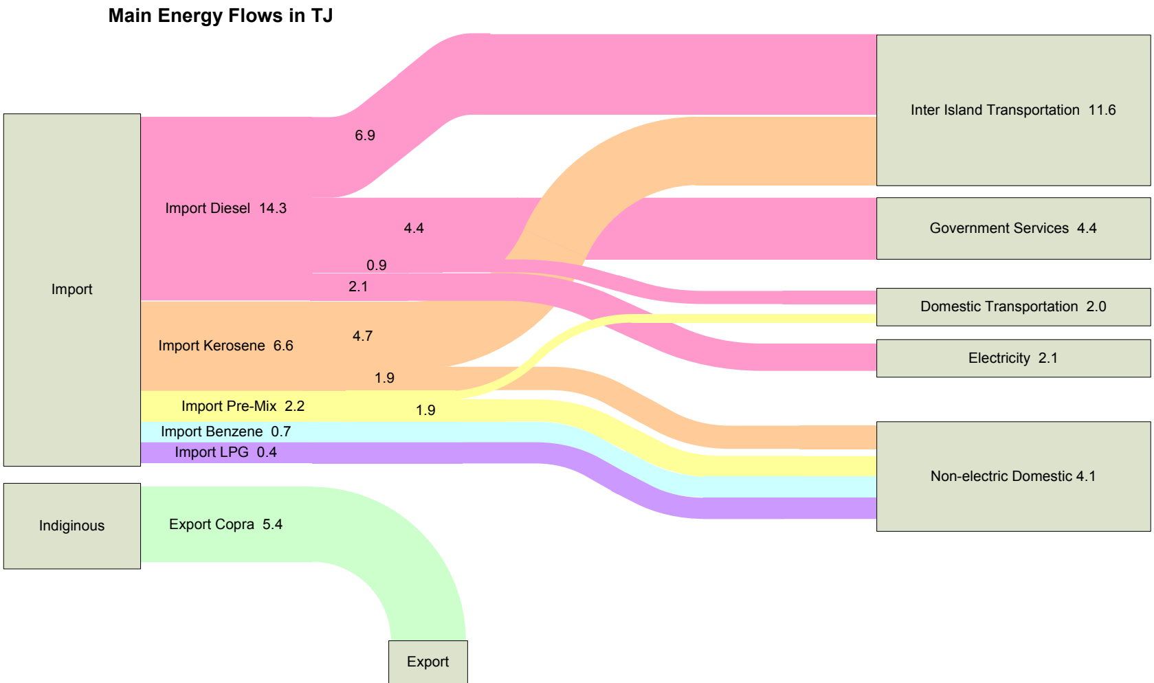
Figure 5.33: Main energy flows on Rotuma in TJ. For comparison, current rates of copra export are added. Copra energy values reflect the energy content of coconut oil that could be produced from the copra.
