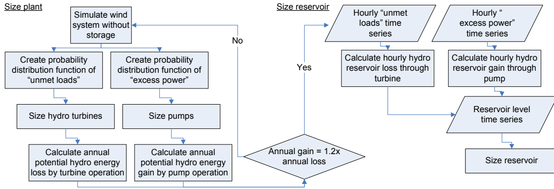
Figure 7.21: Method for modelling of wind power system with pumped storage.
