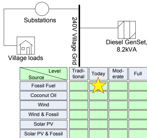
Figure 7.7: Diesel Generation Scheme
